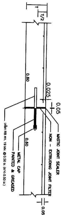
EXPANSION JOINT
